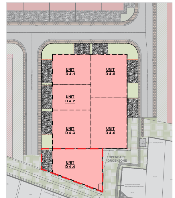
INPLANTINGSPLAN
