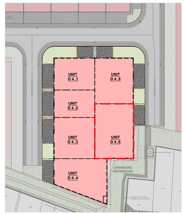
INPLANTINGSPLAN
