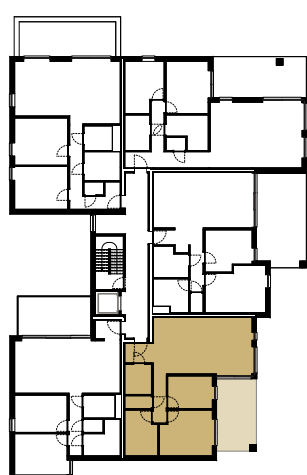
plan verdieping 1
